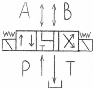
DIRECTIONAL VALVE
